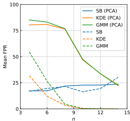
(c) Mean FPR vs n (lower is better)
