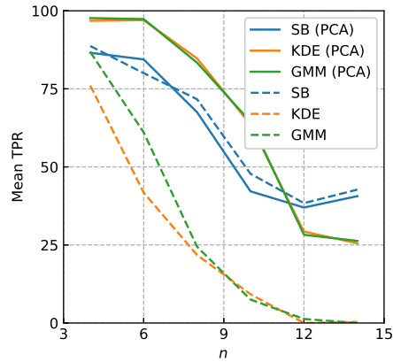
(b) Mean TPR (recall) vs n
