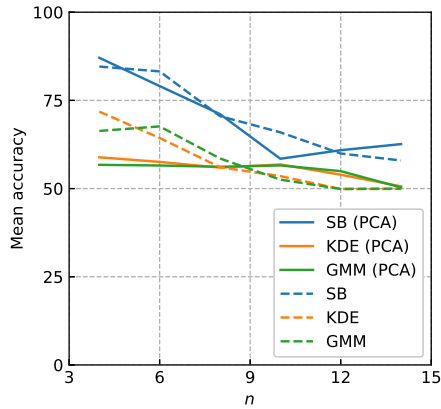
(a) Mean accuracy vs n
